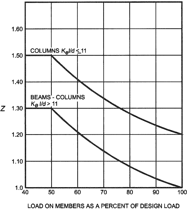
FIGURE 722.6.3(1) LOAD FIGURE
