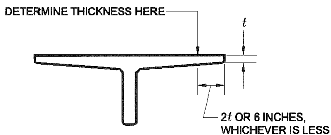
FIGURE 722.2.2.1.2 DETERMINATION OF SLAB THICKNESS FOR SLOPING SOFFITS
