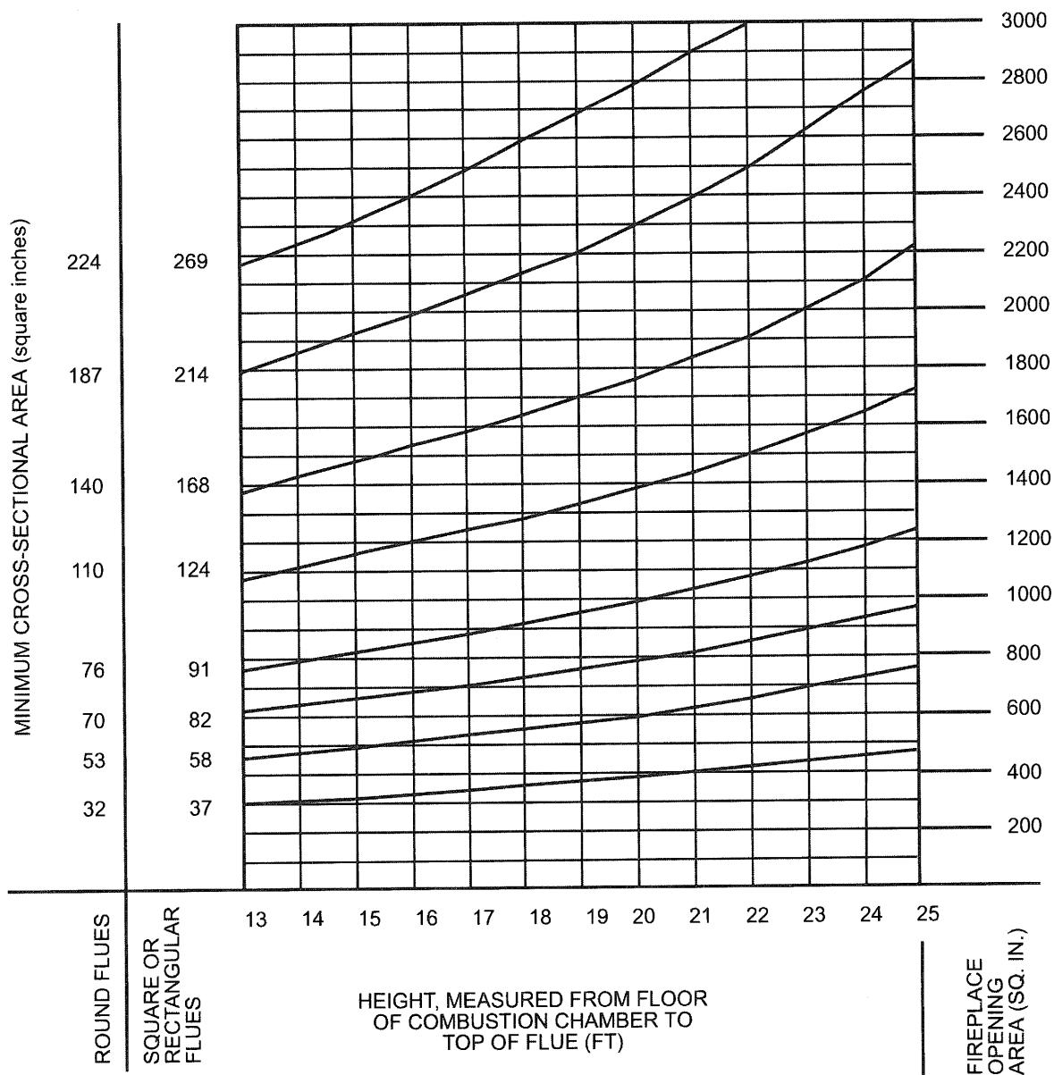
FIGURE 2113.16 FLUE SIZES FOR MASONRY CHIMNEYS
